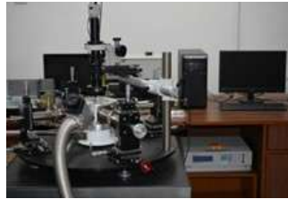
Cryo-Cooled Electrical Probe Station
